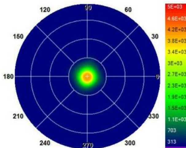
High current, 25 mm LED lamp / reflector assembly with clear lens, log-pseudocolor mapped. \theta grid lines are at 10^\circ intervals.
